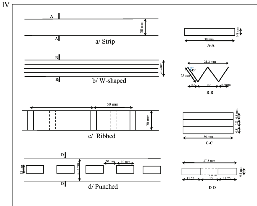
Fig. 3. Geometrical characteristics of reinforcements
