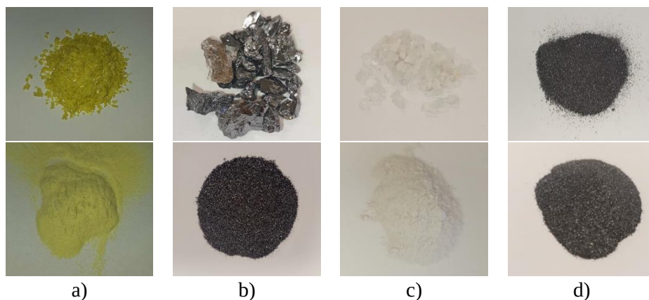
Figure 2. Mineral samples subjected to crushing and classification to prepare feed for flotation a) sulphur, b) silicon, c) fluorite, d) galena, (Błaszczów, 2025)
