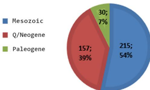
Fig. 2. Distribution of sampling in individual aquifer complexes
