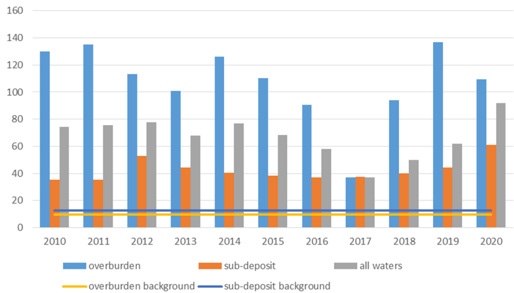
Fig. 6. Average sulfate concentration [mg/dm 3 ] in waters pumped for 10 years
