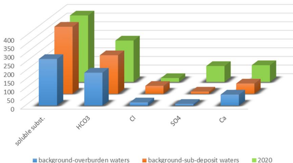
Fig. 4. Average concentration [mg/dm 3 ] of basic ions of water pumped by
