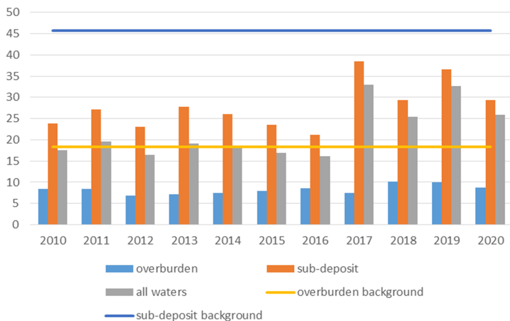
Fig. 5. Average concentration [mg/dm 3 ] of basic ions of water pumped by Szczerców Field wells after 20 years of operation
