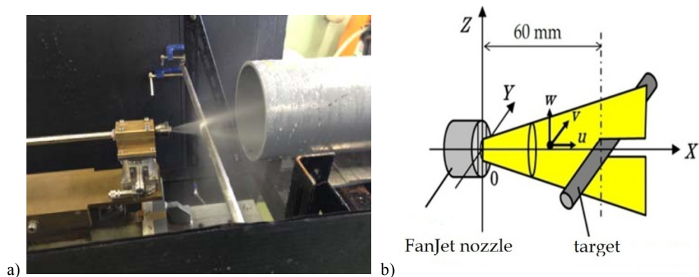
Fig. 3. Research setup for simulation of hydrodynamics occurring in a hydro-jetting mill: general view (a), schema of work zone (b)
