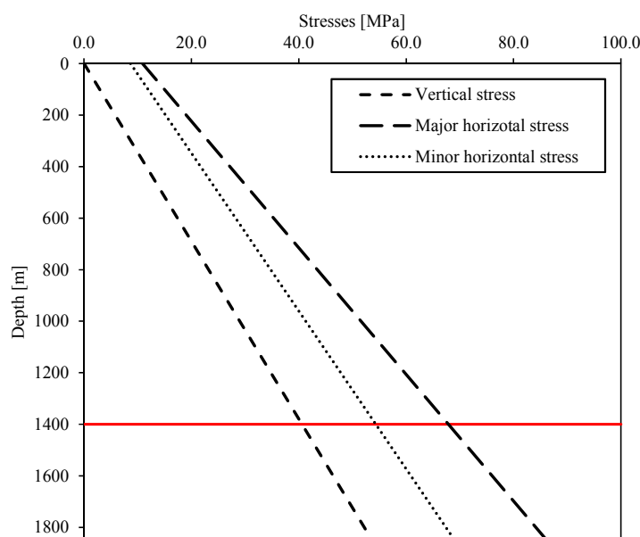
Fig. 3. Stress tensor components vs. depth (red line represents the depth below which the calculation was performed)
