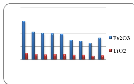
Fig. 2. Chemical analysis distribution of TiO 2 and Fe 2 O 3 against different size fractions
