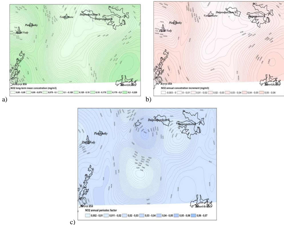
Fig. 3. Spatial distribution of time-series parameters of \text{NO}_2 content in atmosphere of Dnipropetrovsk region for 2009–2014: a – average value of concentration ( \text{mg}/\text{m}^3 ), b – average annual increment of concentration ( \text{mg}/\text{m}^3 ), c – concentration annual periodic component
