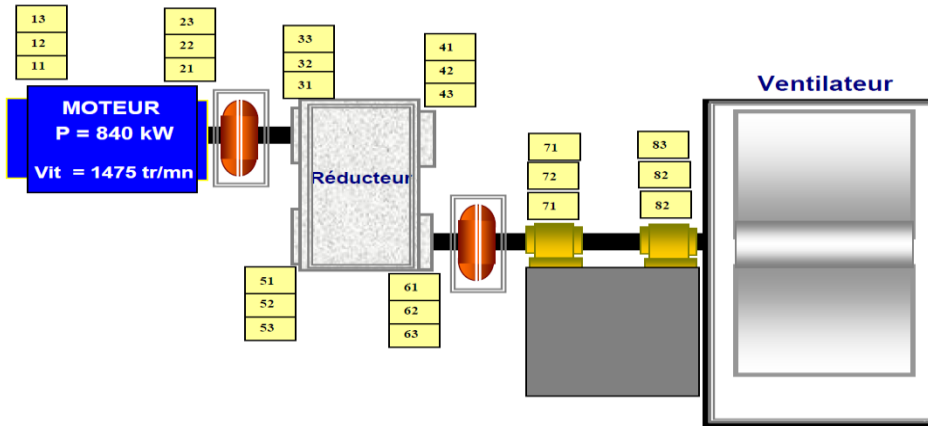
Fig. 5. Block diagram of the fan dispositive
