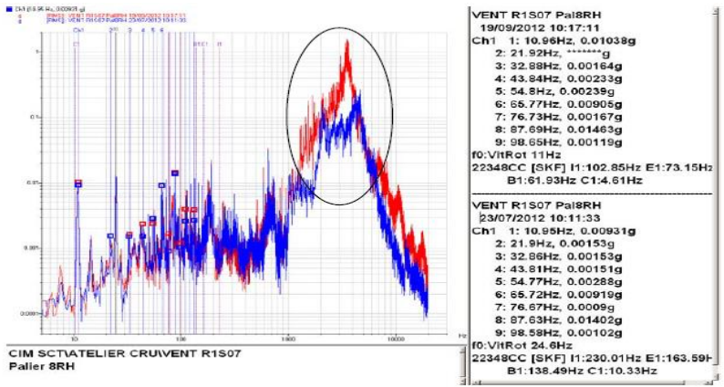
Fig. 8. Spectral analysis in September 2012
